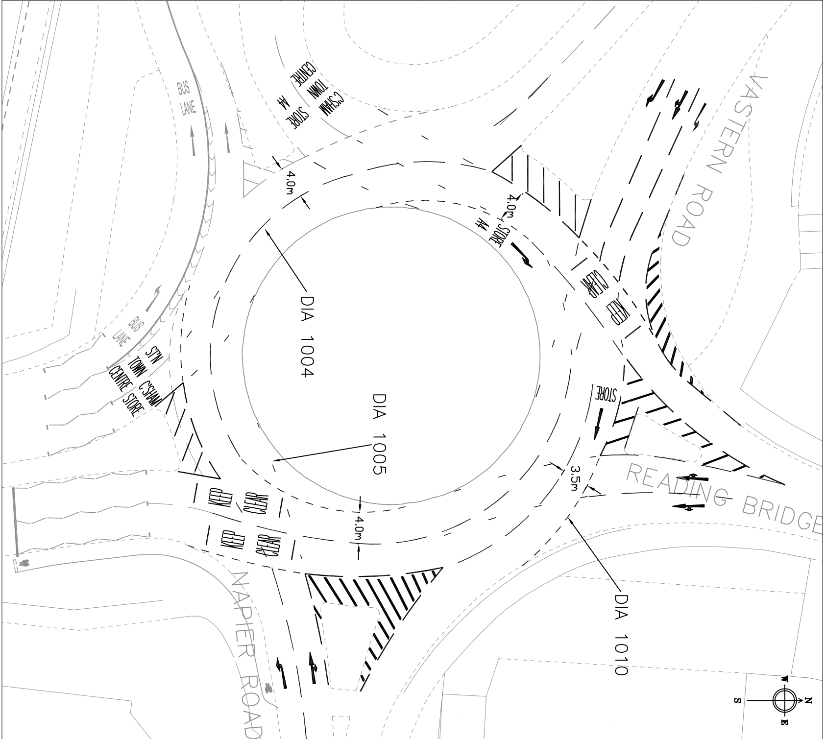
PROPOSED LAYOUT
