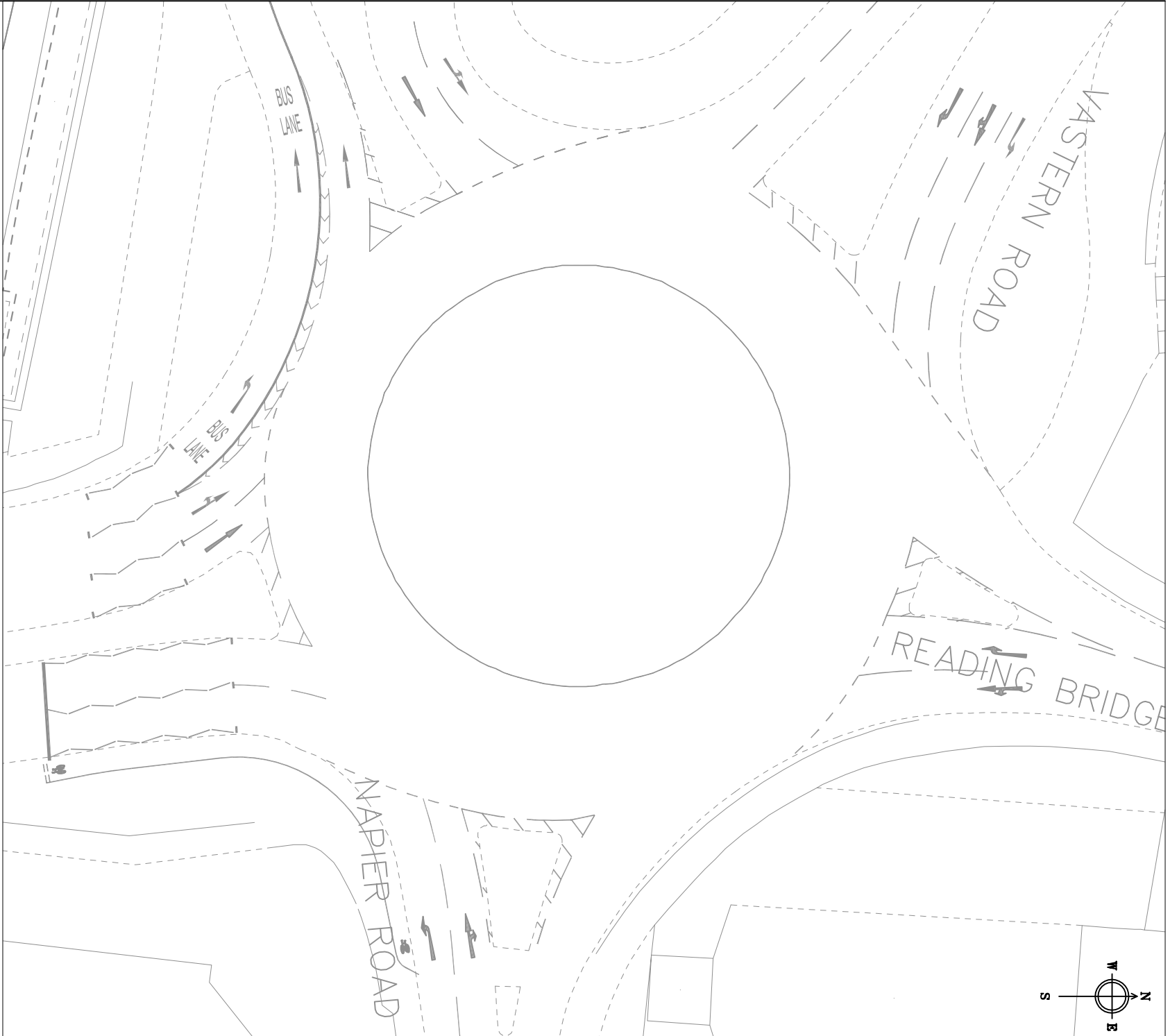
EXISTING LAYOUT
