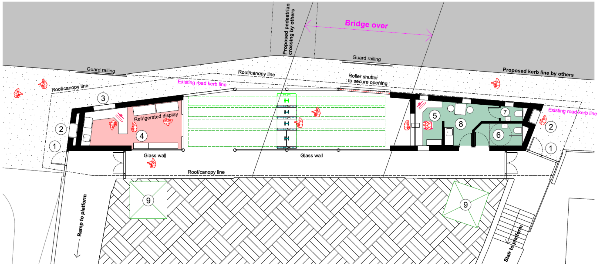
Figure 2 - Oxford Road Entrance - Proposed Station Building Layout
